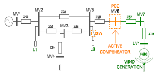
Fig. 1. Study case power system
