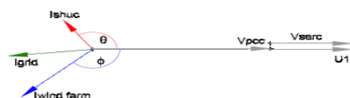
Fig. 3. Phasor diagram of UPQC
