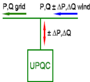
Fig. 7. Power buffer concept
