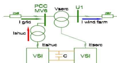
Fig. 2. Block diagram of UPQC
