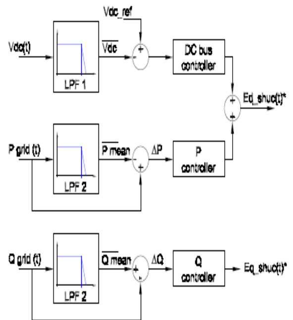
Fig. 6. Shunt compensator controller
