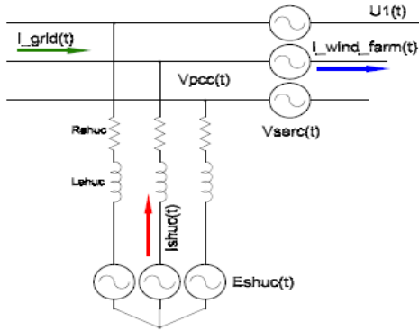
Fig. 4. Power stage compensator model. AC Side
