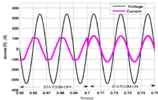
Fig. 9. Supply Voltage and Current at PCC.
