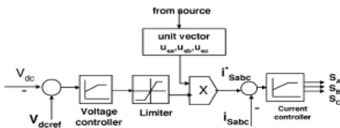
Fig. 3. Control system scheme.
