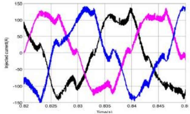
Fig. 5. Three phase injected inverter Current.
