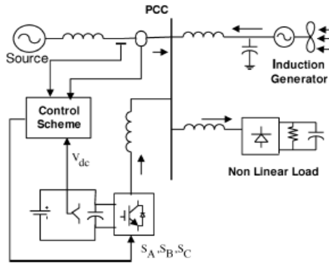
Fig. 2. System operational scheme in grid system.
