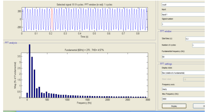
Figure. 9 THD
