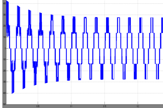
Figure. 7 Five level output Multilevel Inverter without filter
