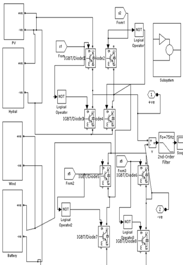
Figure 5 Matlab/Simulink model of Micro grid
