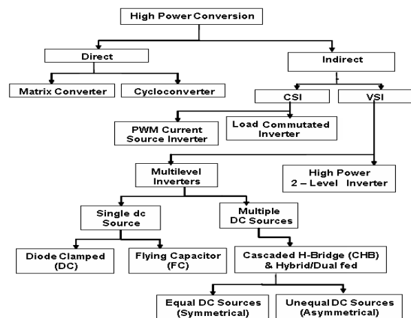
Figure 2 Classification of High power Converters
