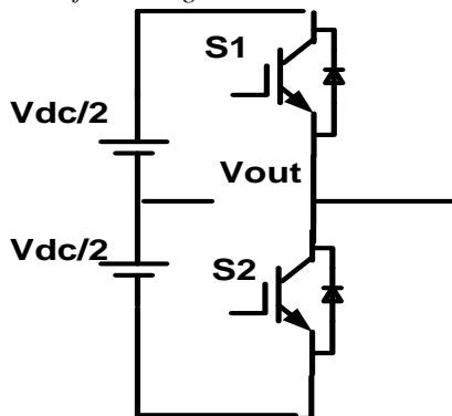
Figure 3 Half Bridge
