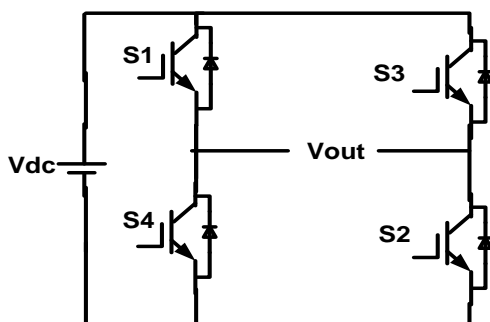
Figure 4 Full H-Bridge
