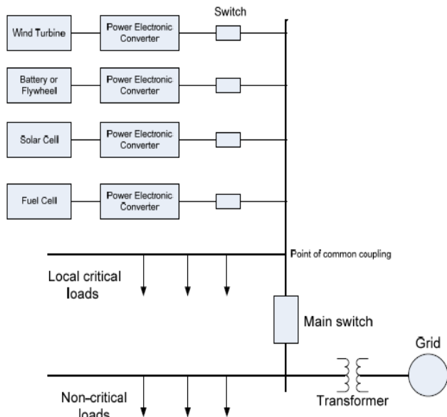
Fig. 1. A Schematic Diagram of a Micro grid
