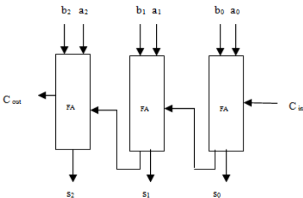
Fig.1: Three Bit Ripple Carry Adder
