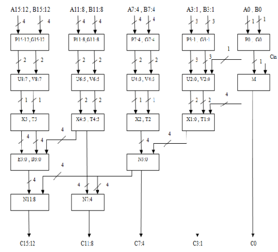
Fig.4: 16-bit Efficient Ladner-Fischer Adder
