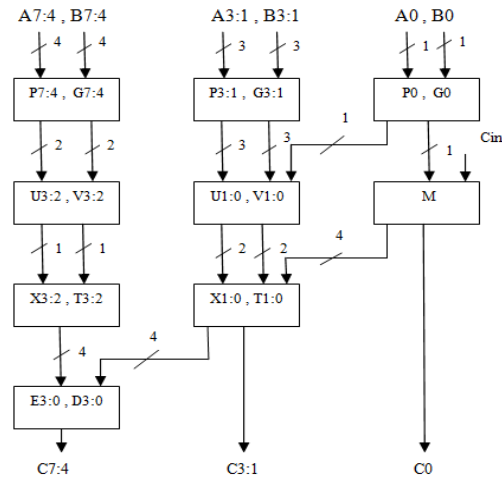
Fig.3: 8-Bit Efficient Ladner-Fischer Adder
