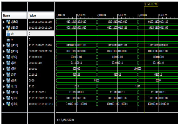
Fig.5: 16-Bit Efficient Ladner-Fischer Adder Simulation Waveform
