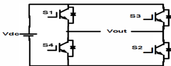
Fig2.4: Circuit of the single cascaded H-Bridge Inverter
