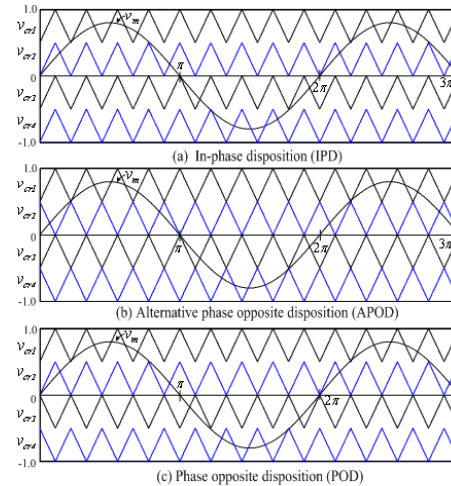
Fig. 4.12 Wave form of Level Shifted PWM
