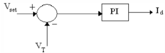
Fig2.2: PI control for reactive power compensation
