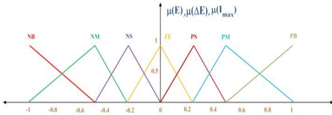
Fig 3.3:Membership functions for Input, Change in input, Output.
