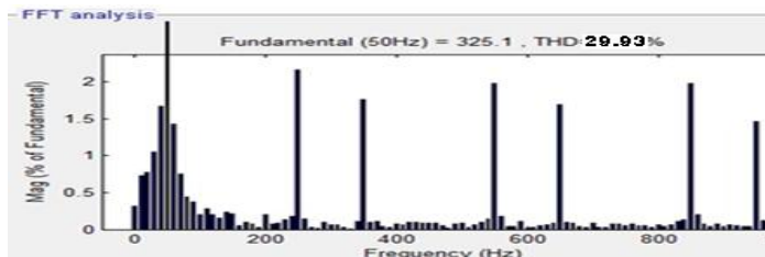
Fig4.7:Harmonic spectrum of phase-a source current with out DSTATCOM
