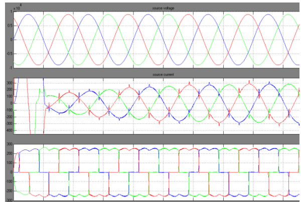
Fig4.3:Source voltage, current and load current with D-STATCOM
