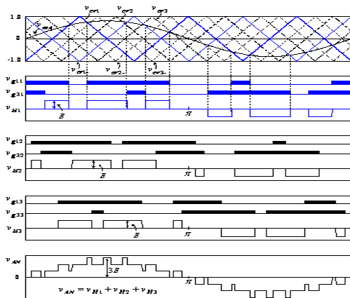
Fig. 4.11 Wave form of Phase Shifted PWM
