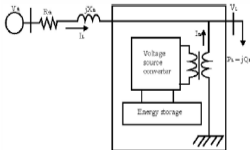
Fig 2.1: Schematic Diagram of a D-STATCOM
