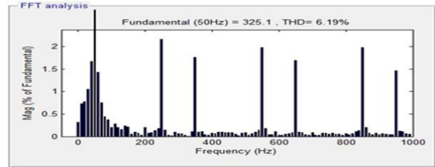
Fig4.8: Harmonic spectrum of phase-a source current with DSTATCOM
