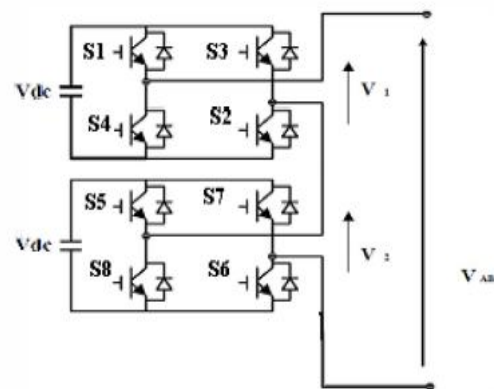
Fig2.5: Block diagram of 5-level CHB inverter model
