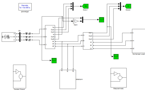
Fig4.1: Matlab/Simulink power circuit model for D-STATCOM
